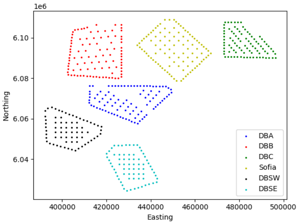
Figure 3: Turbine layouts modelled for large DBS turbine scenario.
